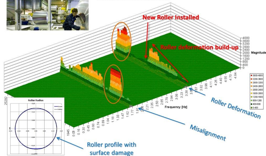
M621 Roller Speed Frequency vs Time
